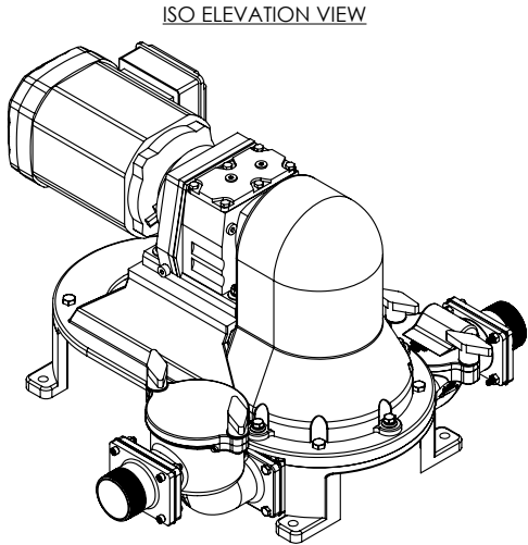
ISO ELEVATION VIEW
