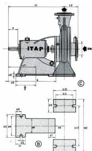
Pump Measurements in mm
