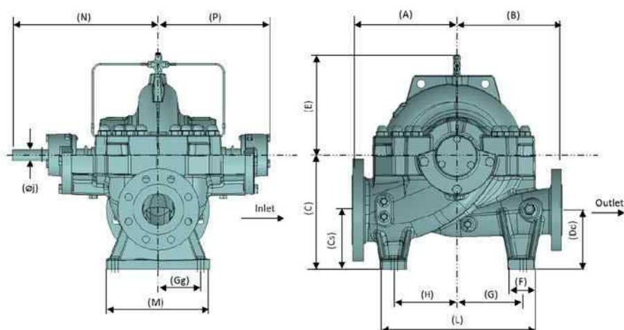
Pump Dimensions
